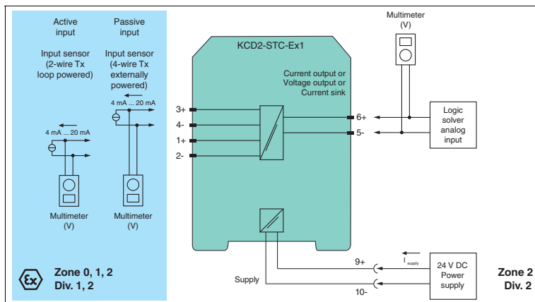
Figure 4.1 Proof test set-up KCD2-STC-(Ex)1(.SP)
