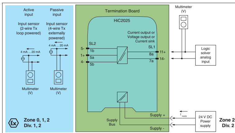
Figure 4.2 Proof test set-up for HiC2025
