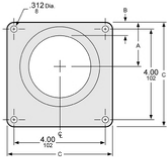
A/L Hub Mounting Dimensions
