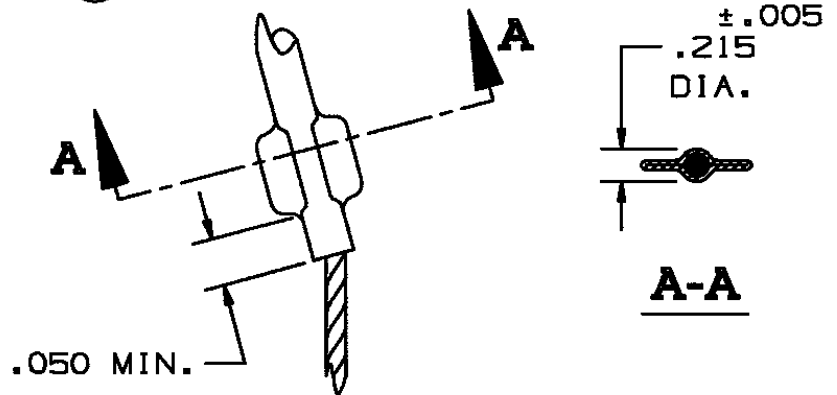
CRIMP DETAIL 2 PL.
