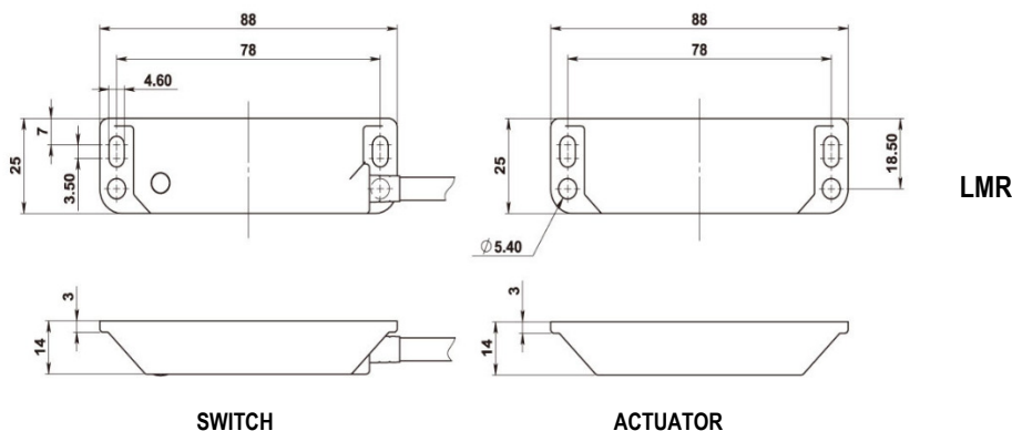
SWITCH
