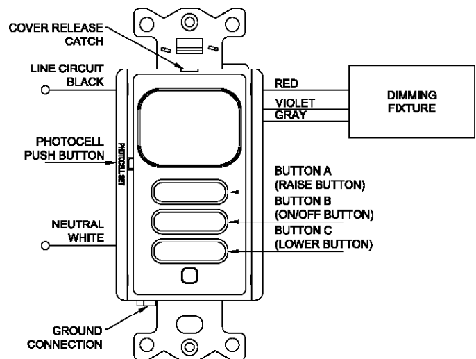
FIGURE 1 - WIRING DIAGRAM
