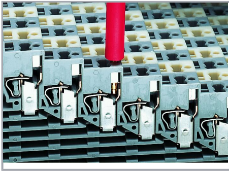
Special test contact for step-down test plug; from 4 mm socket to 2 mm plug; max. 42 V
