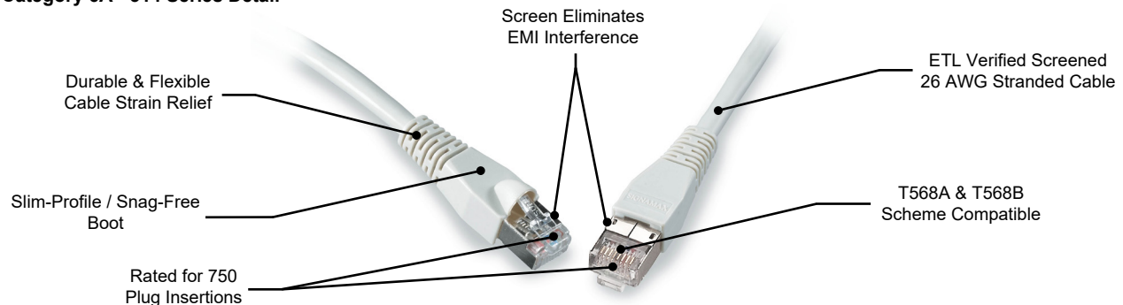
Figure 3: Category 6A - 314 Series Detail
