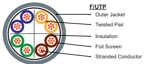
Figure 2: Cable Structure
