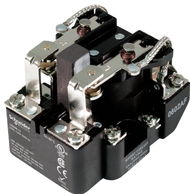
199 Series Relay
