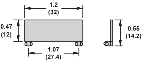
16-750/788FT-1 ID Tag/Label
