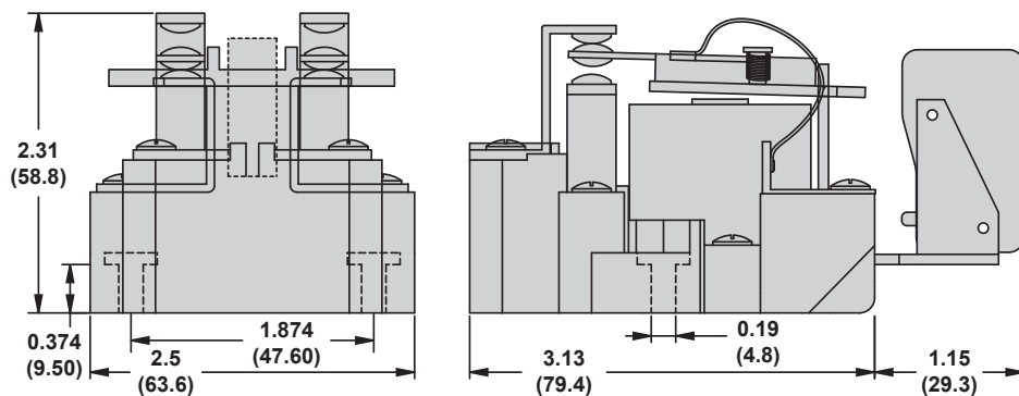
DPDT—Long Base (shown with optional auxiliary switch)
