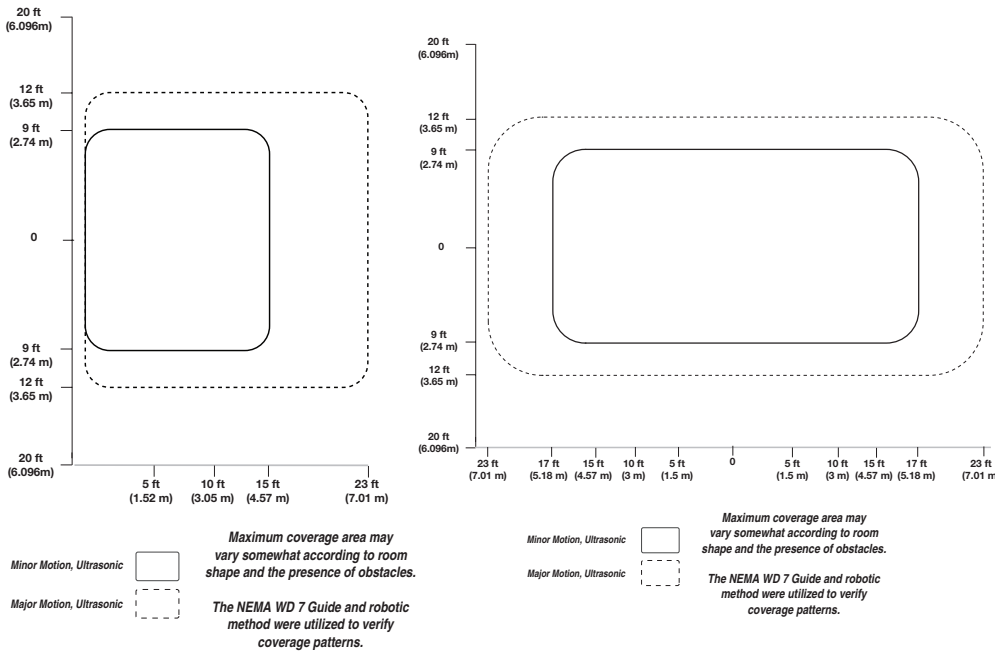
OAC-U-0501-R Coverage Diagram
